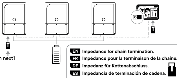
with one nx interface in the communication bus
